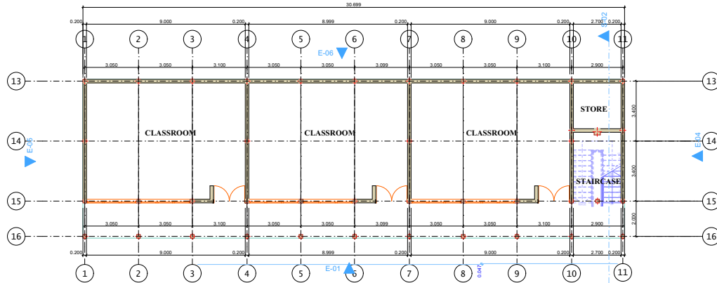
THE GROUND FLOOR PLAN & TYPICAL FIRST AND SECOND FLOOR
