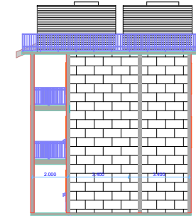
LEFT END ELEVATION
